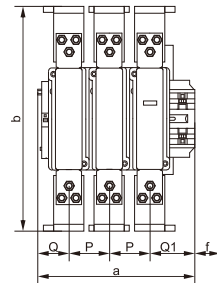
Installation Dimension
