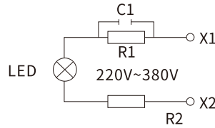
Anti-interference type
